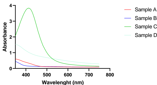
Fig. 8 Spectrophotometric sweeps of nanoparticle synthesis: (A) Distilled water, extract and NaOH, (B) Silver nitrate, (C) Silver nitrate, extract and NaOH, (D) Extract and silver nitrate
