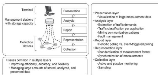
Fig. 1 Sub-classifications of monitoring operations. Reproduced from [5]
