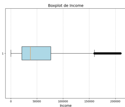
Figura 2: Boxplot de la Variable "Income"
