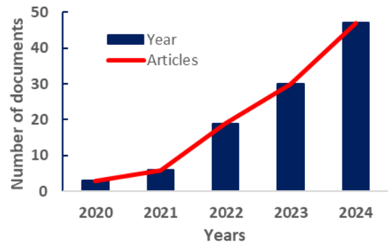
Fig. 2 Annual scientific production in Scopus and WoS.
