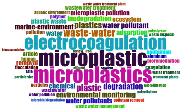
Fig 3. Most popular keywords
