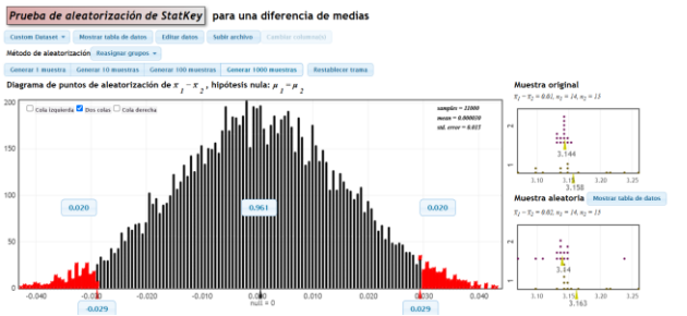
Fig. 7 Hypothesis test for the difference in means of travel speeds of mothers with children
