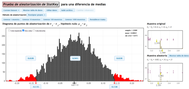
Fig. 6 Hypothesis test for the difference in means of pedestrian travel speeds with motor disabilities.
