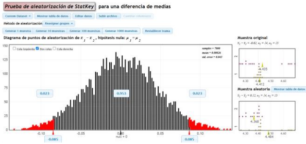
Fig. 5 Hypothesis test for the difference in means of pedestrian travel speeds
