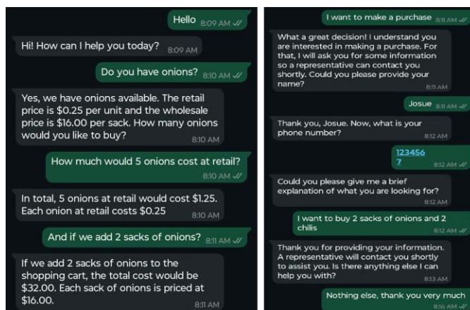
Fig. 3 Chatbot behavior in response to questions related to products and purchase intentions.
