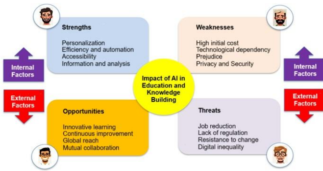
Fig. 2 SWOT Analysis
