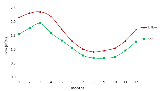
Fig. 9 Ecological and reference flows (ANA) of the Paron station.
