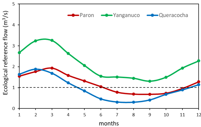
Fig. 8 Ecological reference Flow Curves.
