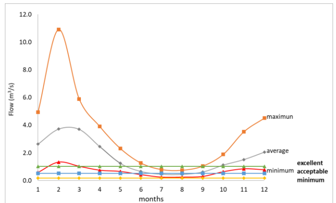
Fig. 7 Ecological Flow Curves - Queracocha Station.
