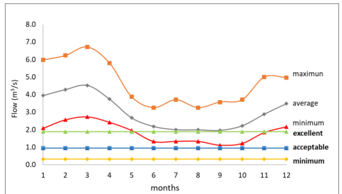
Fig. 6 Ecological Flow Curves - Llanganuco Station.
