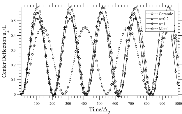
Fig.10 Nonlinear Center Deflection u_2 of Transient Analysis FGM Beam (IFSDT)
