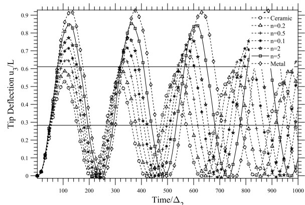
Fig.7 Linear Tip Deflection u_3 of Transient Analysis FGM Beam
