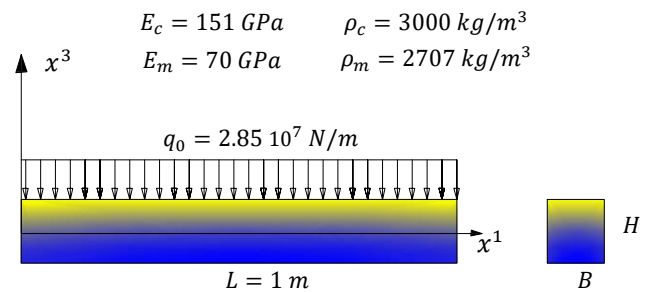
Fig. 6 Geometric properties of the FGM beam
