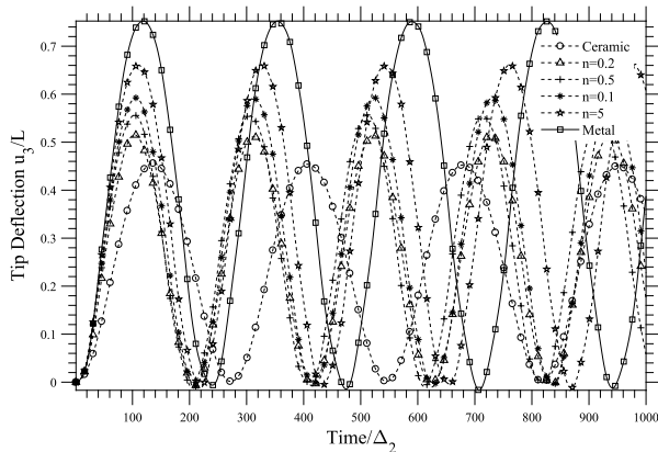
Fig.8 Nonlinear Tip Deflection u_3 of Transient Analysis FGM Beam
