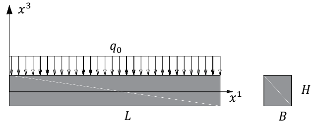
Fig.01 Geometric properties of the beam
