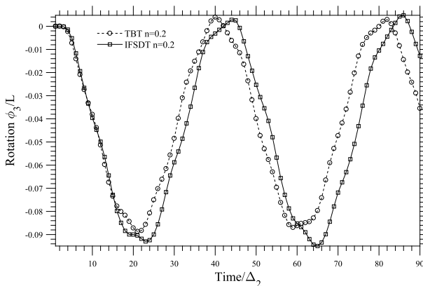
Fig. 4 Rotation \phi_3 of FGM Beam (Linear Response)
