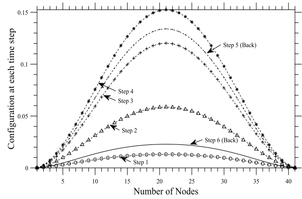
Fig. 5 Configuration at time step of C-C Beam (Linear Response)
