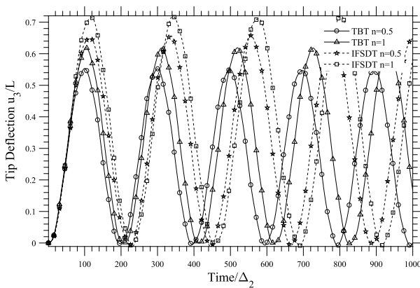
Fig.9 Nonlinear Tip Deflection u_3 of Transient Analysis FGM Beam (TBT vs IFSDT)
