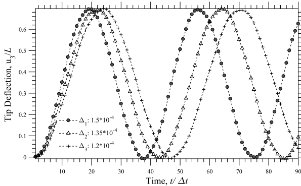
Fig. 3 Different Time Increments of C-F (Linear Response)
