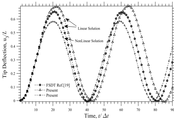
Fig. 2. Transient Analysis of an isotropic cantilever beam
